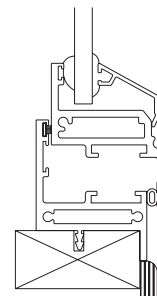
Hinged Unit
